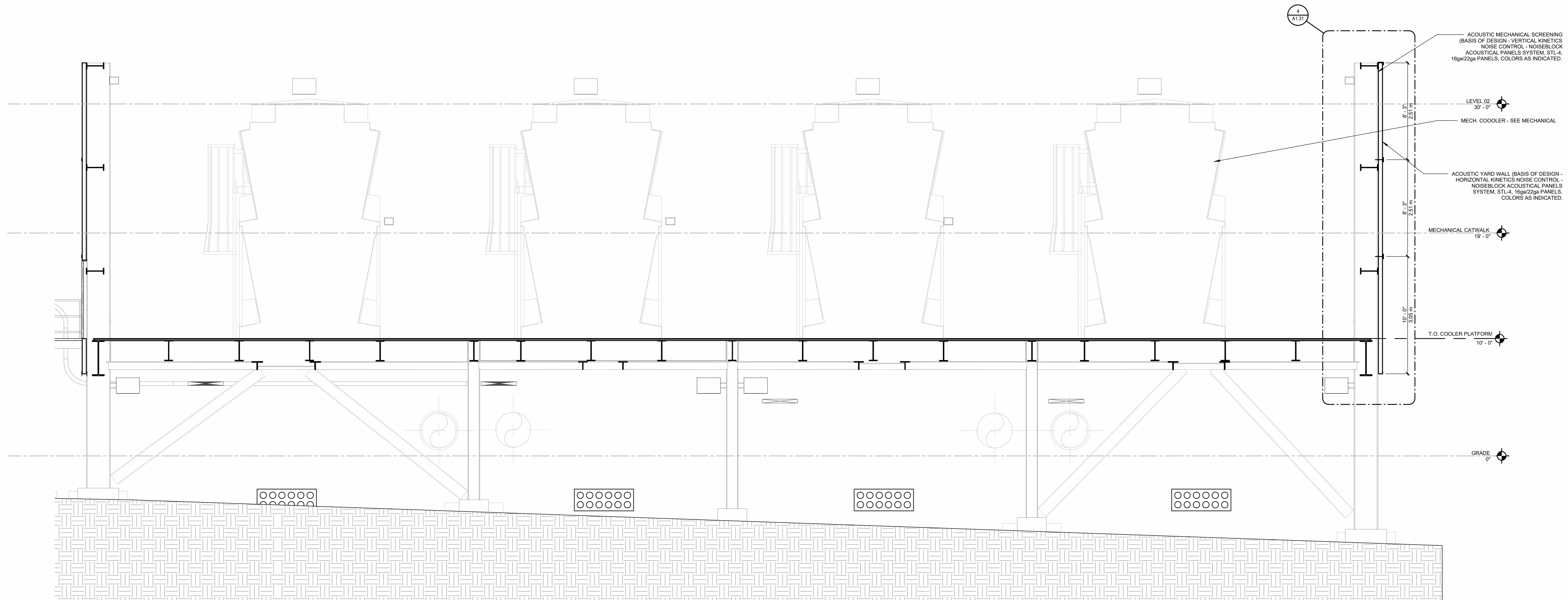
4 MECH COOLER PLATFORM SECTION - 2 1/4" = 1'-0"
